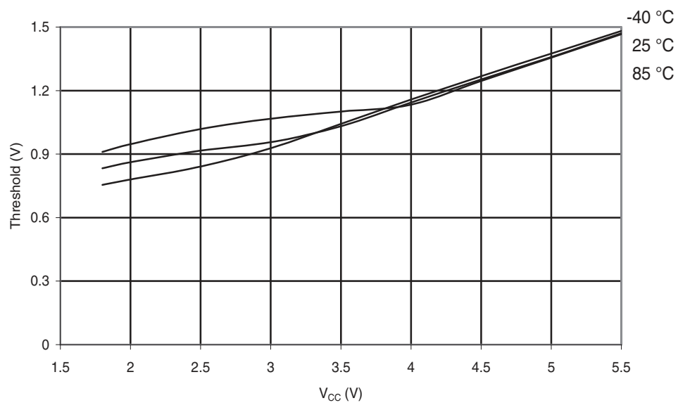
Figure 31-122. ATmega88A: Reset Input Threshold Voltage vs. V_{CC} ( V_{Ith} I/O Pin read as '1')
