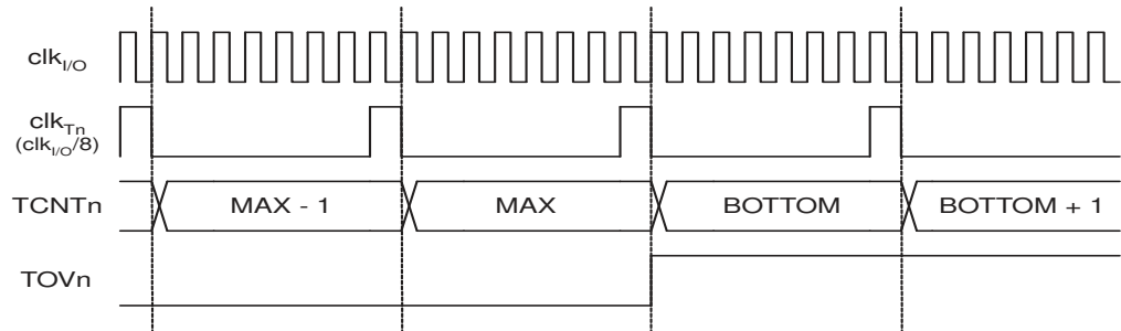
Figure 18-9. Timer/Counter Timing Diagram, with Prescaler ( f_{\text{clk}_{I/O}/8} )
