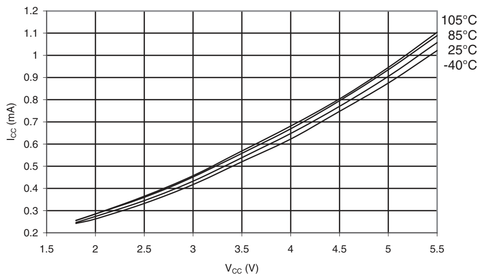
Figure 34-4. ATmega168PA: Active Supply Current vs. V_{CC} (Internal RC Oscillator, 1MHz)
